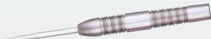
25005 22G Length: 47.0mm Diameter: 7.2mm
