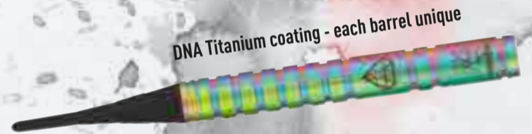
23245 18G IAN WHITE 70% TUNGSTEN Length: 48.3mm Diameter: 6.2mm
